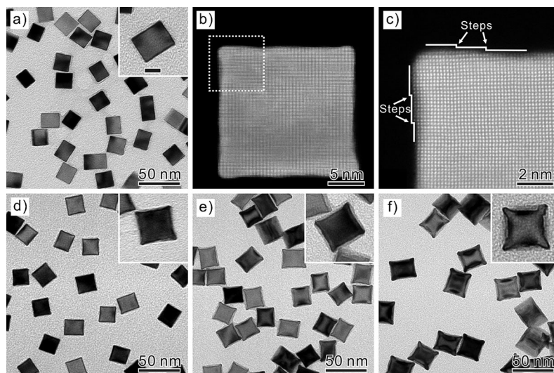
Figure 2. TEM images of Pd-Rh core-frame, concave nanocubes prepared using the standard procedure after different volumes of \text{Na}_3\text{RhCl}_6 solution in EG ( 2.5\text{ mg mL}^{-1} ) had been added into the reacting system: a) 1.0 , d) 2.0 , e) 4.0 , and f) 6.0\text{ mL} . b), c) High-resolution HAADF-STEM images of a single Pd-Rh nanocube shown in (a) and the region marked in (b). The scale bar in the first inset is 10\text{ nm} , and applies to all other insets.
